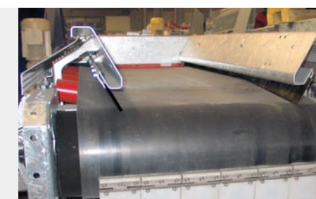
* Load hopper and skirtboard
